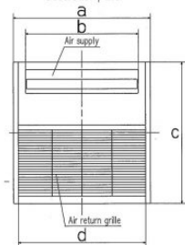
Decorative panel
