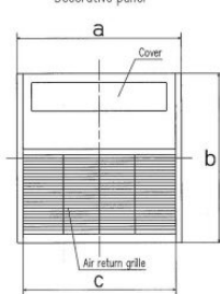
Decorative panel
